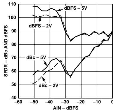
Figure 9. Single Tone SFDR ( f_{IN} = 1.5 MHz, V_{CM} = 2.5 V)
